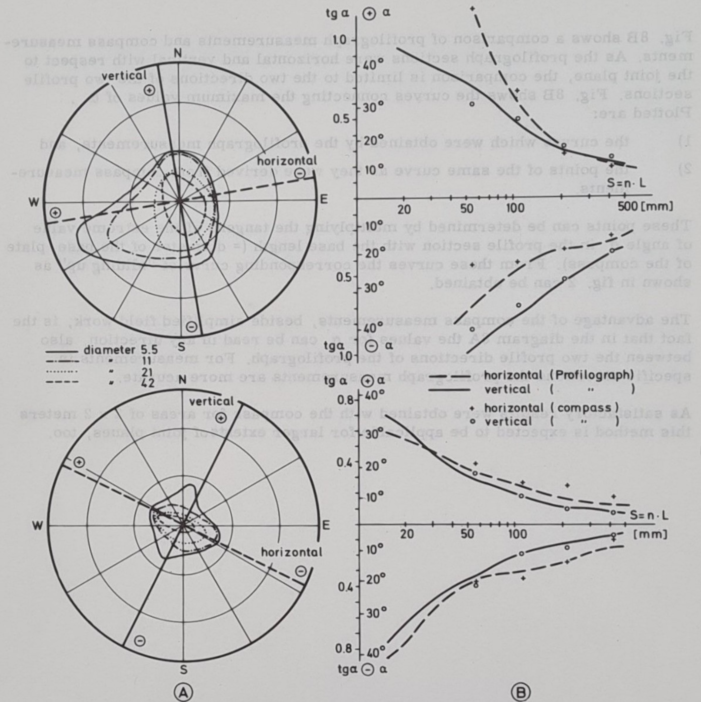
Fig. 8: (A) Curves of the maximal scattering from different base plates of the compass. (B) Comparison from compass measurements and profilograph measurements by the curve of the "extreme values of \alpha ".
