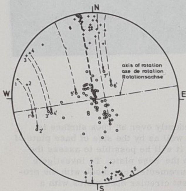
Fig. 5: Rotation of reference plane \diamond in horizontal position. The poles of joint measurements were also rotated around the same axis. Pole 1 will be after pole 1' etc.
