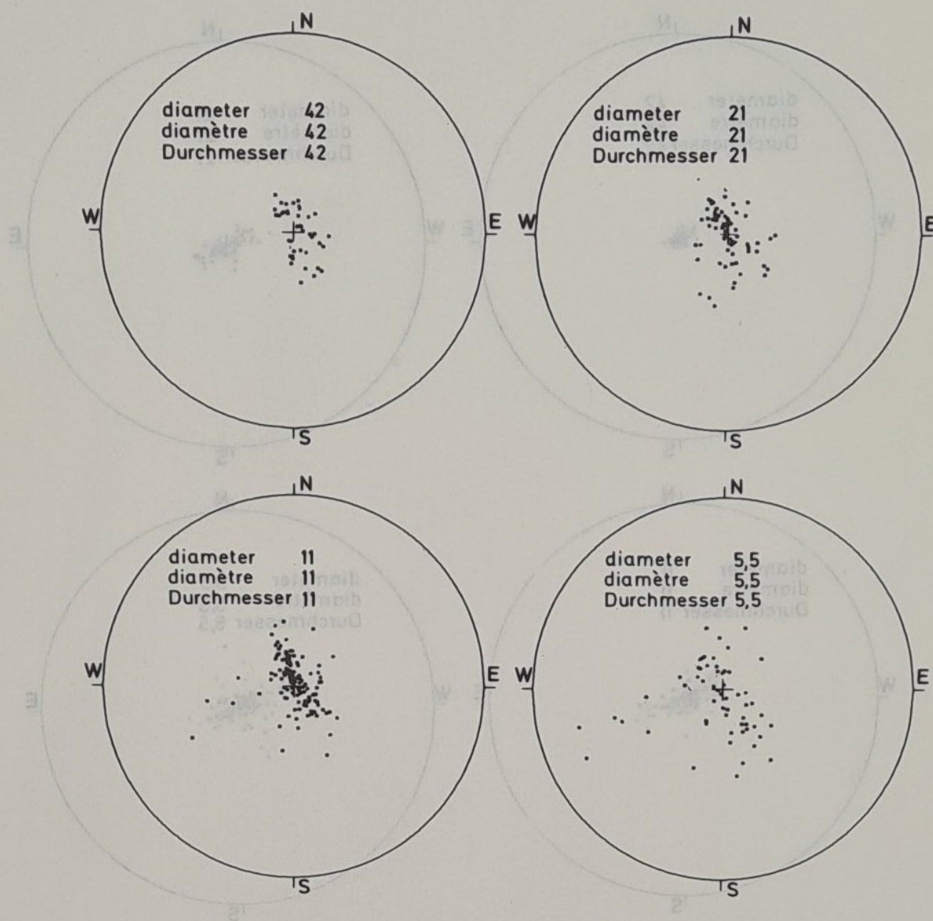
Fig. 6: Rotated pole diagram of fissure 1
